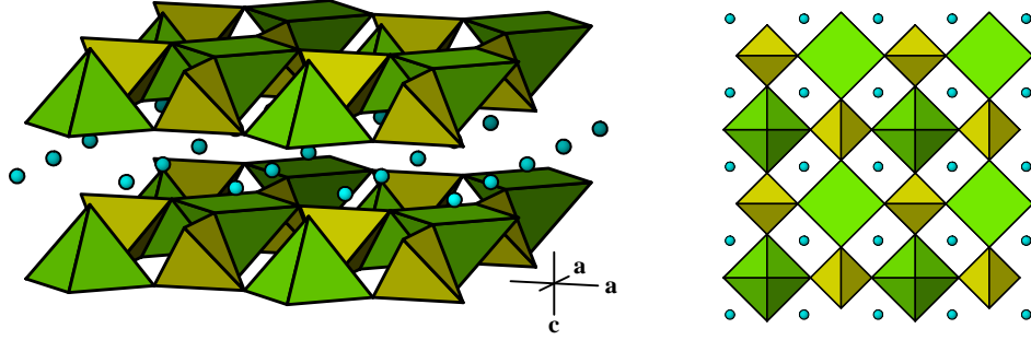
Fig. 1. Perspective view (upper panel) of the crystal structure of \text{Li}_2\text{VOSiO}_4 and projection along [001] (lower panel). The \text{VO}_5 pyramids (large diamonds) share the corners of the basal planes with \text{SiO}_4 tetrahedra (small diamonds). The \text{Li}^+ ions are indicated by circles.
