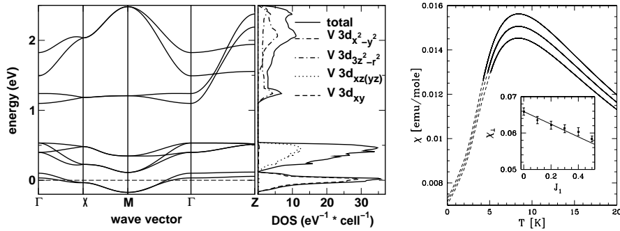
Fig. 2. (Left) Band structure, total and orbital resolved DOS of \text{Li}_2\text{VOSiO}_4 for the V 3d related bands. The Fermi level is at zero energy. (Right) Susceptibility ( \chi , with largest \chi for J_1 = 0 ) for J_2 = 9K , g = 2 and J_1/J_2 = 0, 0.1, 0.2 . The low- T data is obtained from QMC, while the high- T data comes from HTE. The inset shows Ising series expansion calculations for T = 0 , J_2 = 1 .
