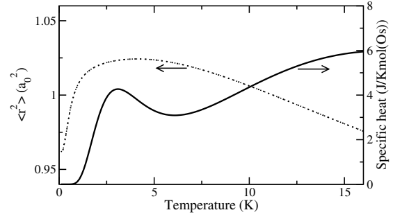
Fig. 3. The calculated specific heat and mean square displacement of K ion as a function of temperature.
