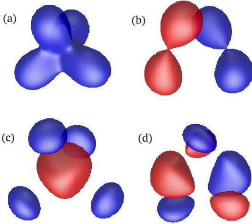
Fig. 2. The lowest energy orbitals ground state singlet (a) and triplet (b) (only one orbital shown), and singlet (c) and triplet (d) (only one representative shown).
