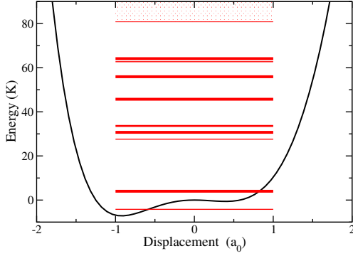
Fig. 1. Single site potential for K ion along (111) direction with the energy levels depicted by horizontal lines. Thickness reflects the degeneracy (from 1 to 3).
