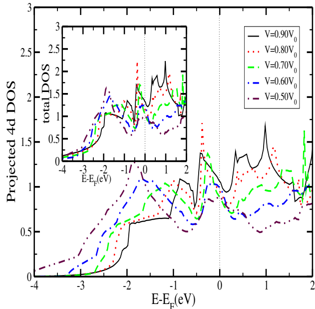
FIG. 1: (Color online) Plot of the total DOS and projected 4d DOS per atom of fcc Y with different volumes. Both the total and the 4d density of states at Fermi level decrease with reduction in volume.
