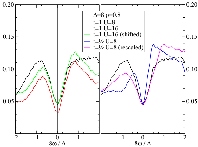
FIG. 3: Scaling of the pseudogap as a function of interaction and hopping. The key observation is that the pseudogap is unchanged when U increases from U = 8 to U = 16 (left panel), and hence the antiferromagnetic exchange J is halved, but has a width which is proportional to t (right panel). The shifting in the third data set is done so as to make the two minima, for U = 8 and U = 16 , coincide. In the last data set the energy axis was rescaled by a factor of two.
