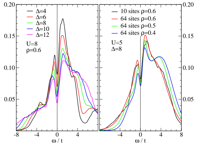
FIG. 2: Evolution of the local spectral density away from half-filling (no Mott gap at \Delta = 0 ). Left panel: A(\omega) as a function of \Delta . \Delta ranges from well below U to well above. The dip in A(\omega) at \omega = 0 becomes deeper as \Delta increases. In the clean limit \Delta = 0 we observe no pseudogap this far from half-filling, in agreement with [3, 4, 5]. Right panel: DQMC results on a 8 \times 8 = 64 site lattice at T = t/6 averaging over 64 disorder realizations. The scale (width) of the pseudogap is largely independent of doping. For \rho = 0.6 the 10-site Lanczos result is also reported. Despite the different cluster size the agreement between the two techniques is excellent.
