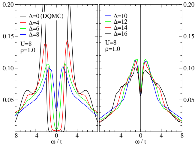
FIG. 1: Evolution of the local spectral density, A(\omega) , at \rho = 1 for U = 8 as a function of \Delta . Left panel: \Delta \leq U . The Mott gap evident for \Delta = 0 and 4 is partially filled in as the randomness increases, so that the value at the Fermi surface, A(\omega = 0) , becomes finite at \Delta = U . Right panel: \Delta > U . A pseudogap survives even for large randomness. The spectra are the average of 1000 independent disorder realizations.
