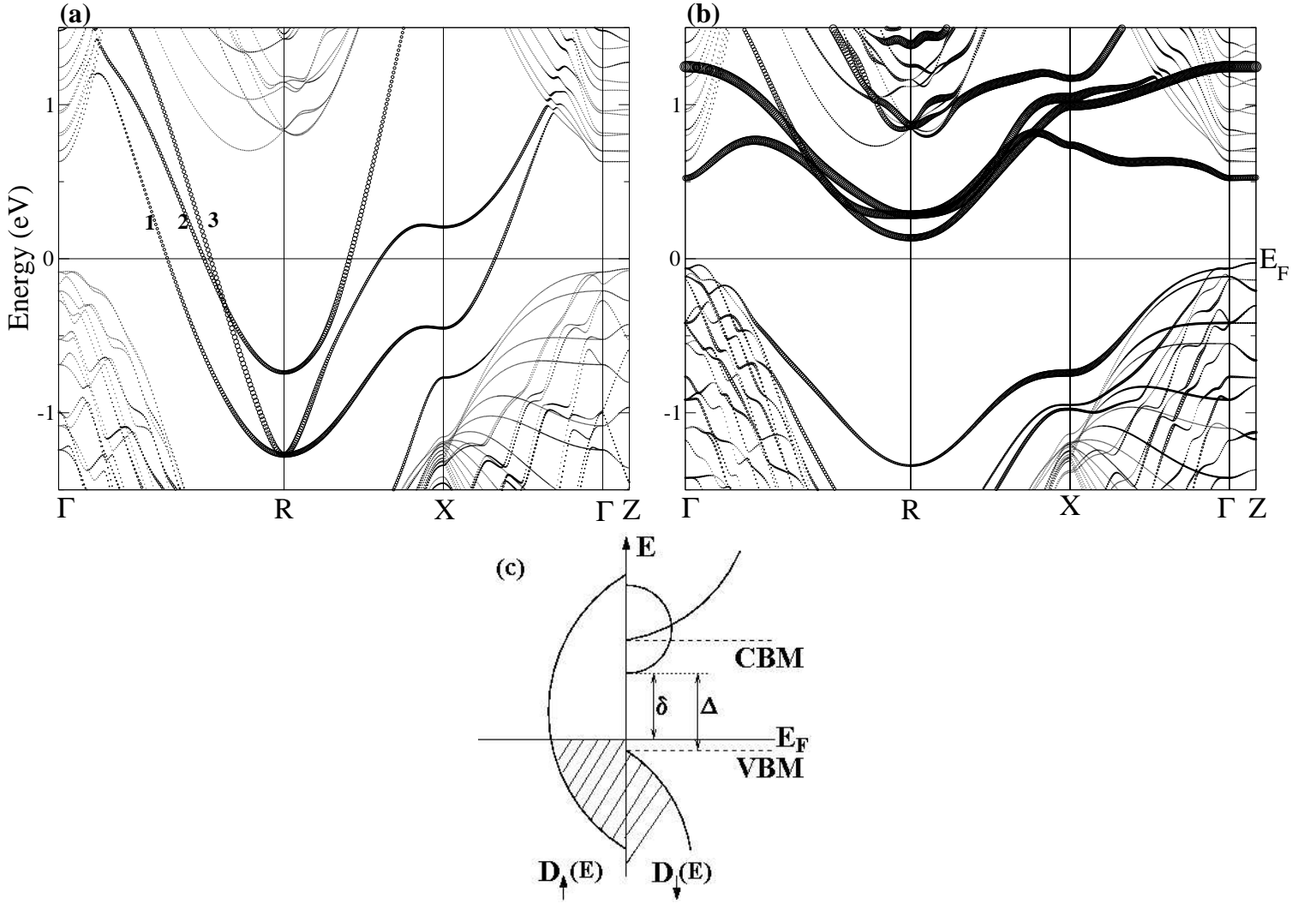
FIG. 3: Calculated band structure along \Gamma -R-X- \Gamma in the k_x - k_y plane and along \Gamma -Z in the k_z -direction, (a) spin up and (b) spin down for Mn \delta -doped in Si. High symmetry points of the Brillouin zone are \Gamma = (0, 0, 0) , R= (1, 1, 0) , X= (1, 0, 0) , and Z= (0, 0, 1) . The size of circles indicates the fraction of Mn d character. The conduction bands are labeled 1, 2 and 3. (c) Schematic diagram of the density of states D(E) in Mn/Si-DFH of the two spin channels near E_F . VBM and CBM are the valence band maximum and conduction band minimum, respectively, of Si crystal for comparison.
