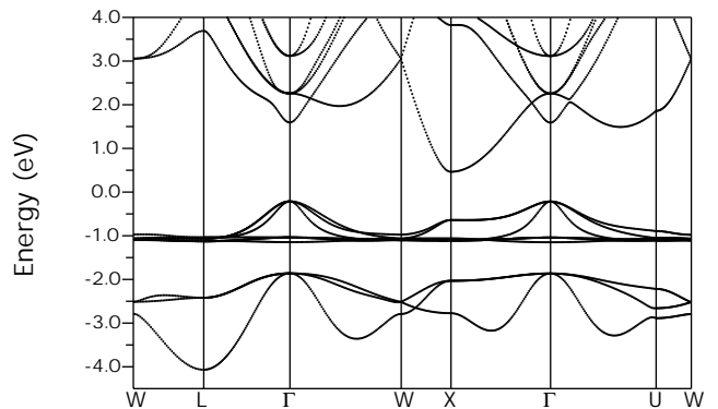
FIG. 4: Majority spin bandstructure of EuSe obtained with U=7 eV at ambient pressure. The valence bands have dominant Se 4p character while the conduction bands are mostly Eu d and s states. The occupied f states are located inside the semiconductor gap.
