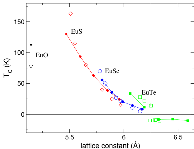
FIG. 3: (color online) The magnetic ordering temperatures calculated for U=6 eV (lines+symbols) compared to the experimental values for EuO [27] and EuS, EuSe, and EuTe [24, 25](open symbols). The negative values indicate Néel temperature. Experimental data for EuO at elevated pressure are not available.
