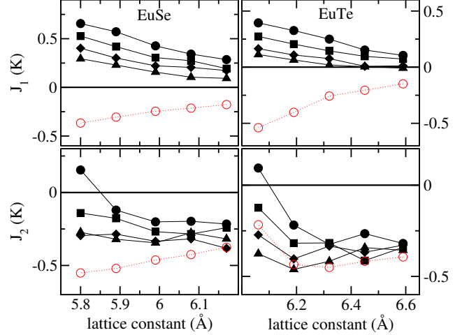
FIG. 2: The same as in Fig. 1 for EuSe and EuTe.
