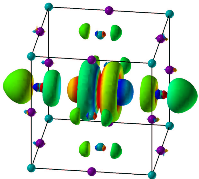
FIG. 5: (color online) The Wannier orbital corresponding to the dispersive f band represented by isosurface of |\phi(r)| . The large lobes on Se sites on the axis of the orbital as well as smaller lobes on the four remaining nearest-neighbor Se sites indicate a rather strong Eu 4f - Se 4p mixing. There are two other symmetry related orbitals on the same site.
