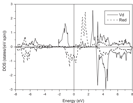
FIG. 3: Density of states plots of the tetragonal double perovskite \text{Sr}_2\text{VReO}_6 in a HMAF state within an LSDA+U scheme with U=5 eV for V and 3 eV for Re, including spin-orbit coupling. Upper (lower) panel shows up (down) spin channel.
