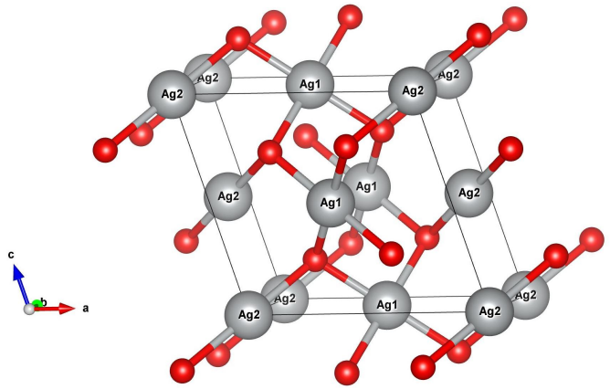
FIG. 1: Crystal structure 17 of monoclinic \text{AgO} . \text{Ag}^{III} sits at the center of a slightly distorted but planar oxygen square, while \text{Ag}^I forms an O-Ag-O linear trimer with its nearest neighbors. Differences in coordination numbers and bond lengths suggest distinct charge states for \text{Ag}^{III} and \text{Ag}^I .
