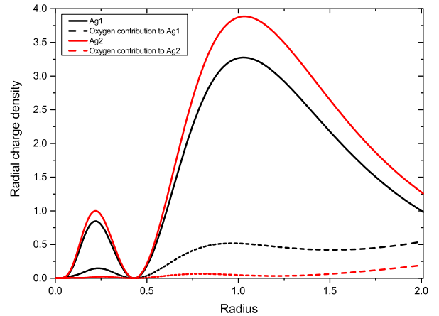
FIG. 4: Black solid line: radial charge densities 4\pi r^2 \rho(r) versus distance from the Ag nucleus, in a.u. Red solid line: sum from the five \text{Ag}^{\text{I}} WFs. Black solid line: sum from four \text{Ag}^{\text{III}} WFs. Dashed lines: corresponding contributions from the O 2p WFs within the Ag spheres. The O WFs make large contributions to the \text{Ag}^{\text{III}} atomic density.
